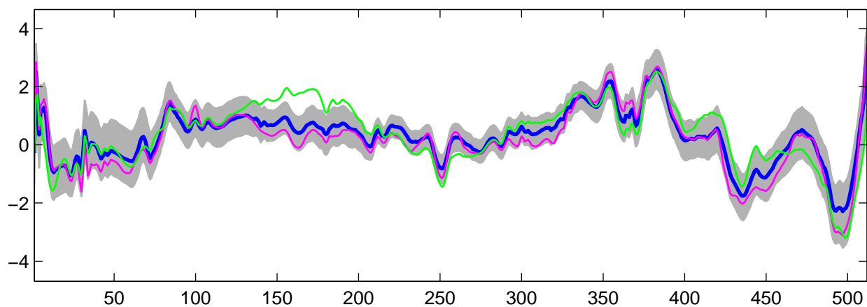
Estimated U_{26}(t) using R-WFMM: t_2 data, run 1
