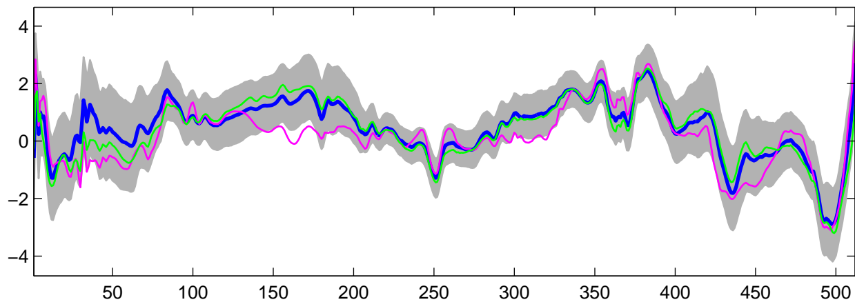
Estimated U_{26}(t) using G-WFMM: t_2 data, run 1
