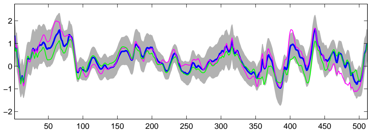
Estimated U_{26}(t) using R-WFMM: t_3 data, run 1
