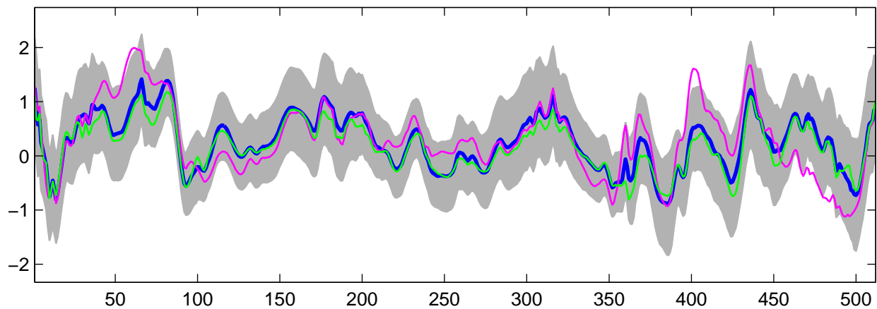
Estimated U_{26}(t) using G-WFMM: t_3 data, run 1
