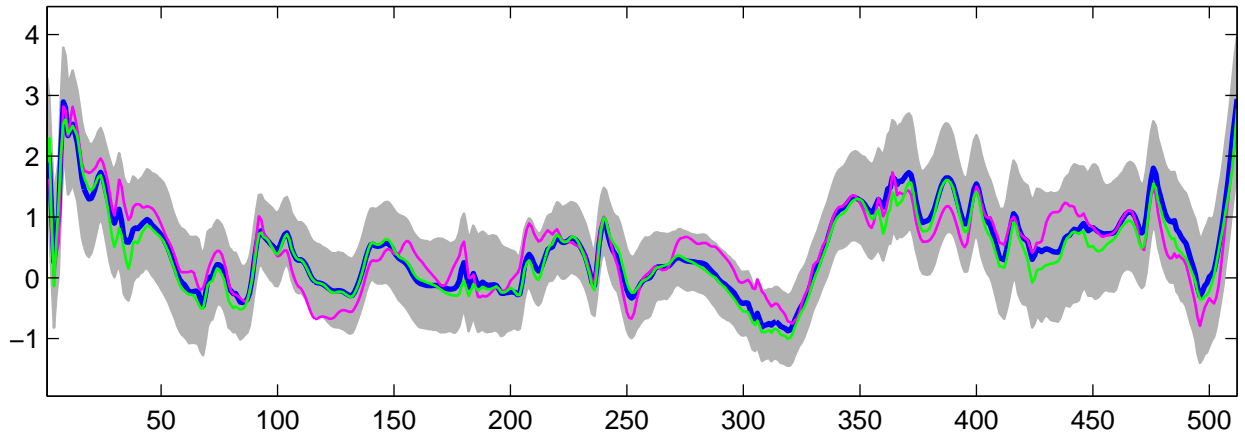
Estimated U_{27}(t) using G-WFMM: Normal data, run 1
