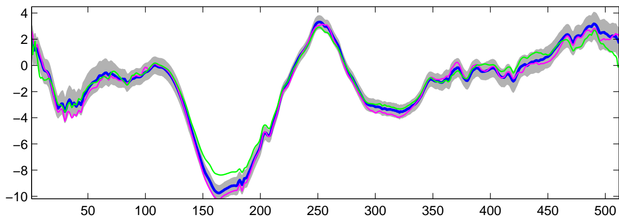
Estimated U_{27}(t) using R-WFMM: t_2 data, run 1
