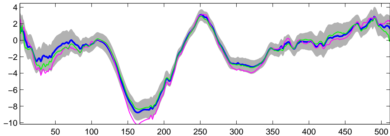
Estimated U_{27}(t) using G-WFMM: t_2 data, run 1
