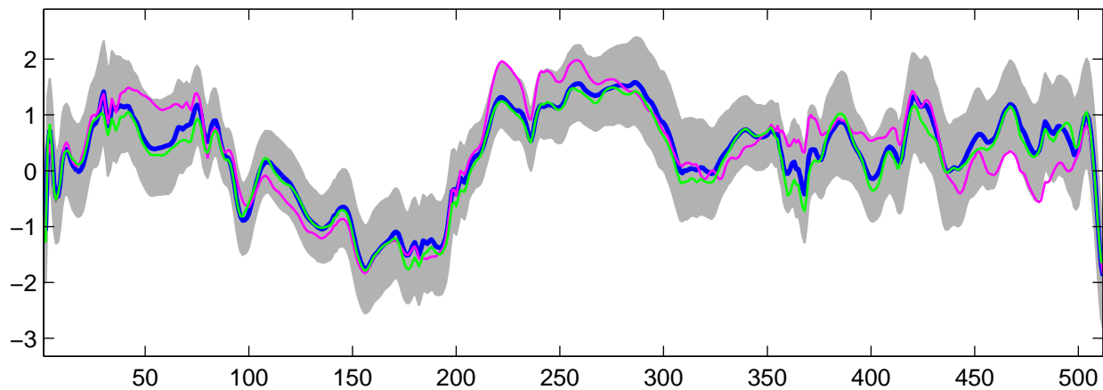
Estimated U_{27}(t) using G-WFMM: t_3 data, run 1
