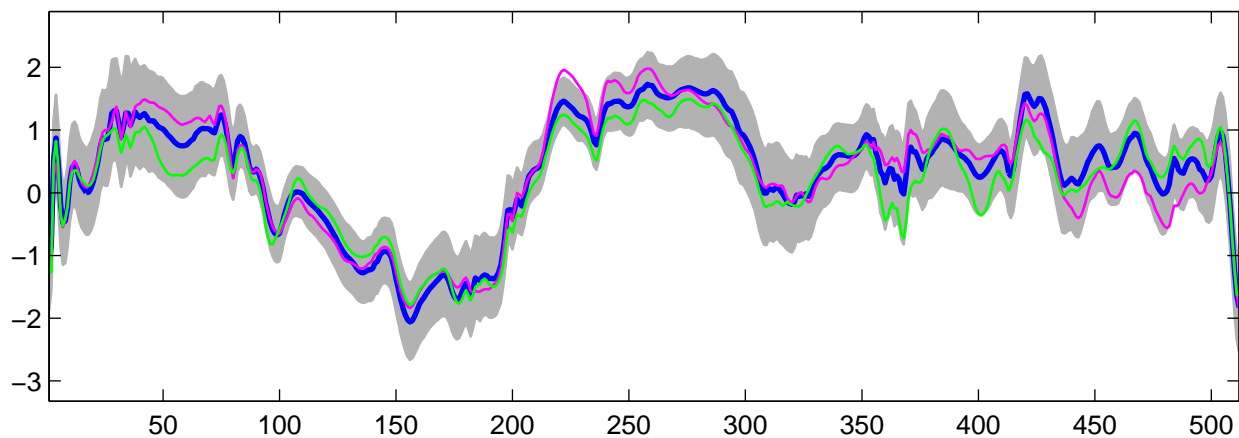
Estimated U_{27}(t) using R-WFMM: t_3 data, run 1
