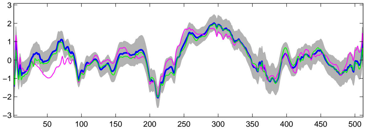
Estimated U_{28}(t) using R-WFMM: DE data, run 1
