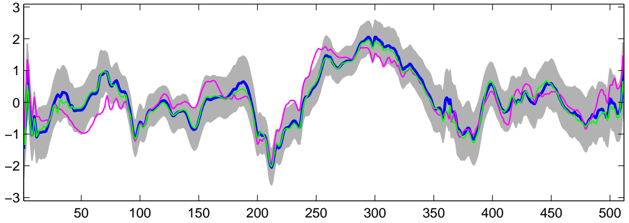
Estimated U_{28}(t) using G-WFMM: DE data, run 1
