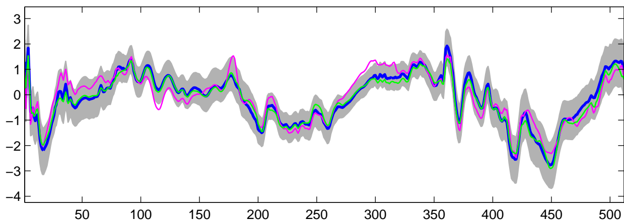
Estimated U_{28}(t) using R-WFMM: Normal data, run 1
