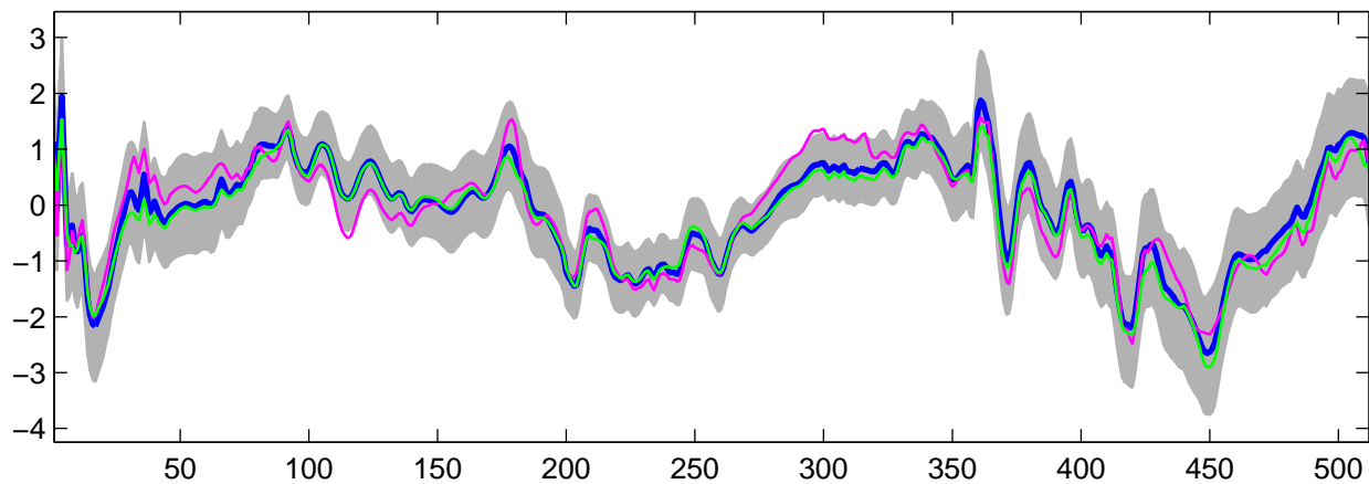
Estimated U_{28}(t) using G-WFMM: Normal data, run 1
