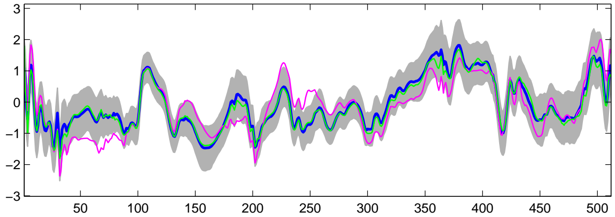
Estimated U_{29}(t) using G-WFMM: DE data, run 1
