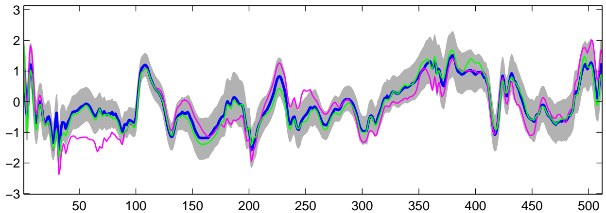
Estimated U_{29}(t) using R-WFMM: DE data, run 1
