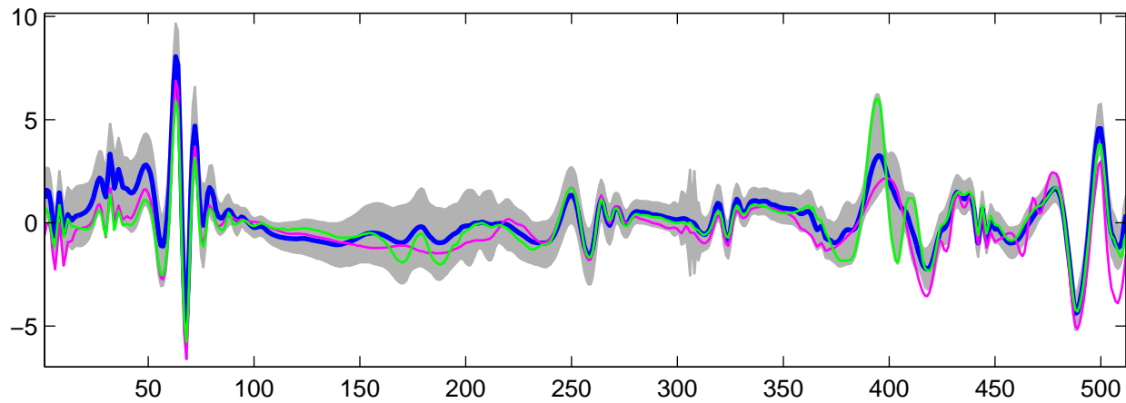
Estimated U_{29}(t) using G-WFMM: t_1 data, run 1
