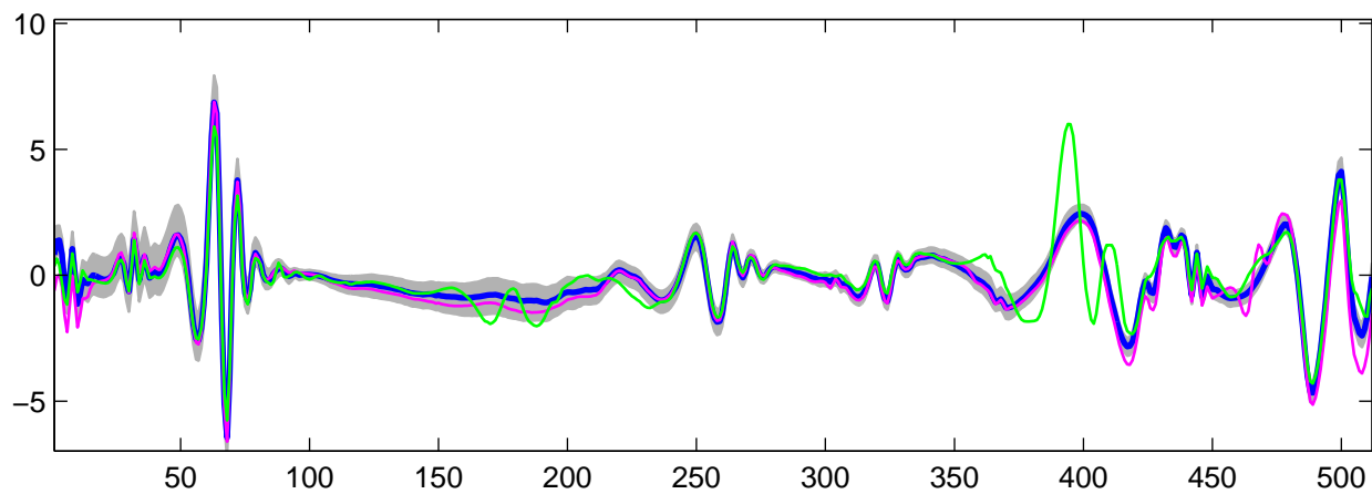
Estimated U_{29}(t) using R-WFMM: t_1 data, run 1
