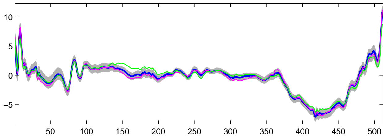
Estimated U_{29}(t) using R-WFMM: t_2 data, run 1
