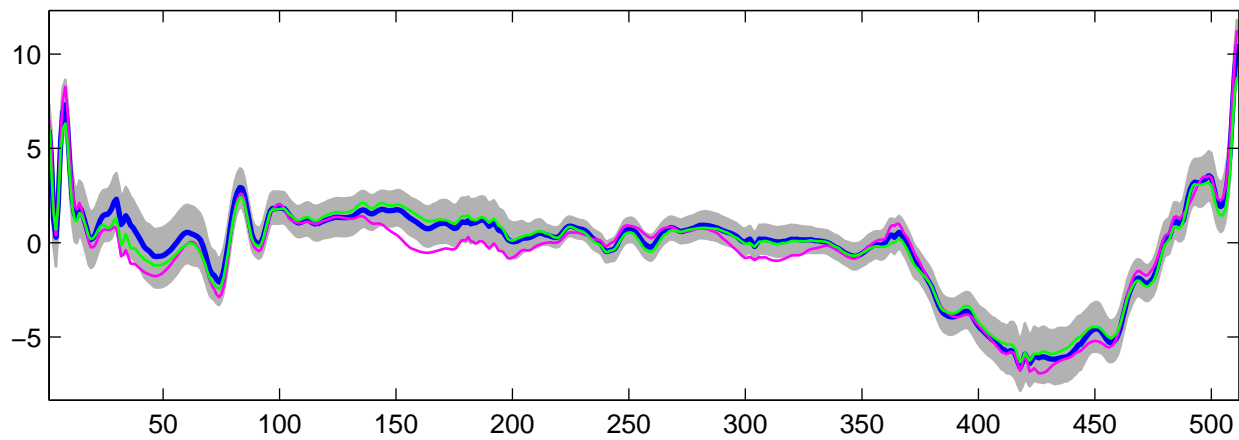
Estimated U_{29}(t) using G-WFMM: t_2 data, run 1
