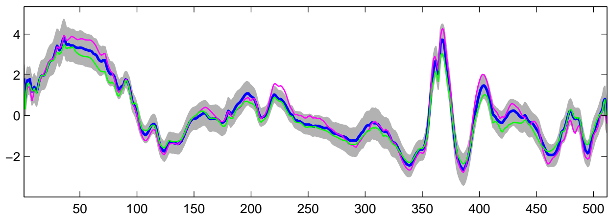
Estimated U_{29}(t) using R-WFMM: t_3 data, run 1
