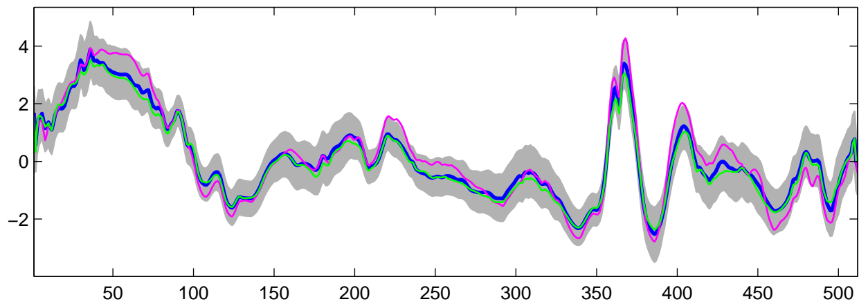
Estimated U_{29}(t) using G-WFMM: t_3 data, run 1
