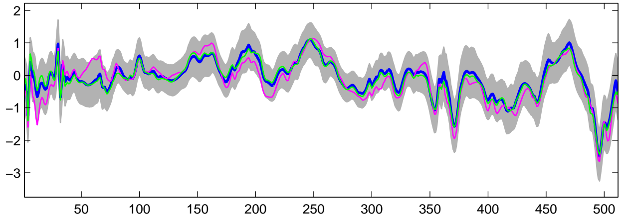
Estimated U_2(t) using G-WFMM: DE data, run 1
