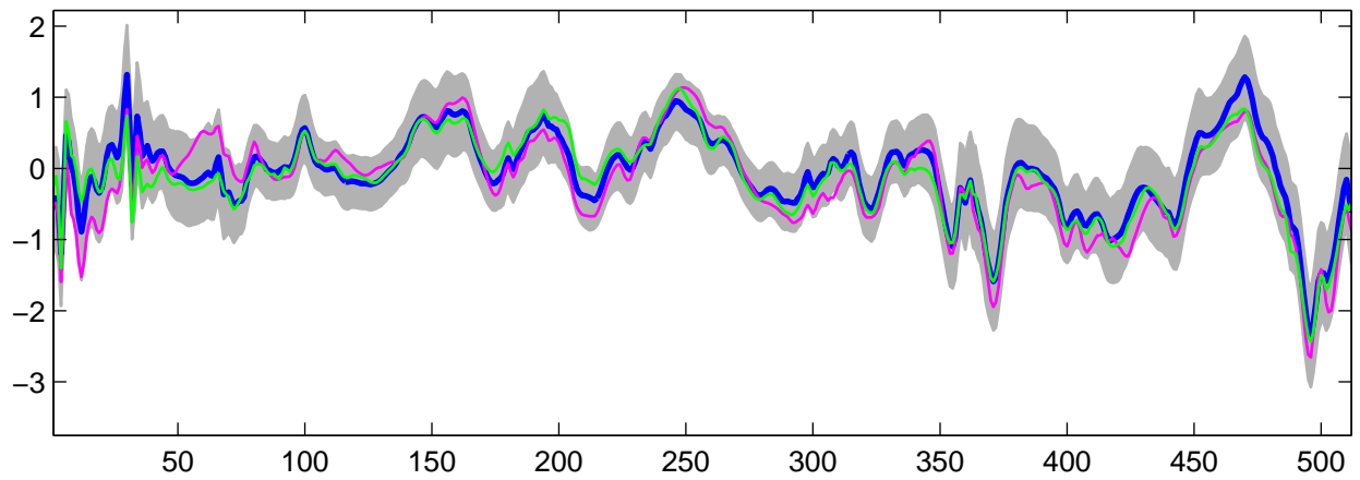
Estimated U_2(t) using R-WFMM: DE data, run 1
