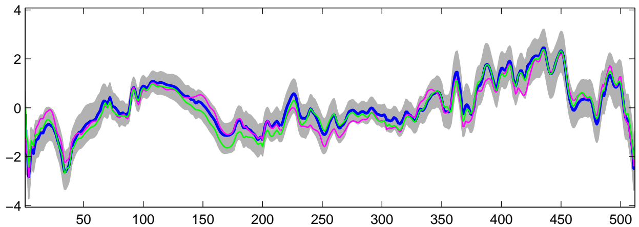
Estimated U_2(t) using R-WFMM: Normal data, run 1
