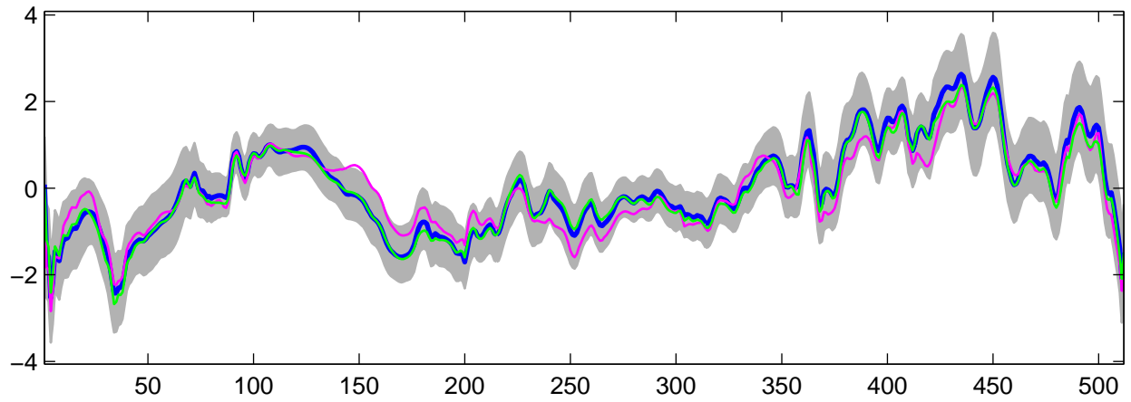
Estimated U_2(t) using G-WFMM: Normal data, run 1
