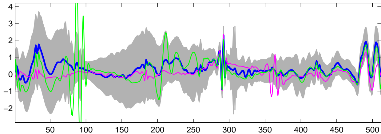
Estimated U_2(t) using G-WFMM: t_1 data, run 1
