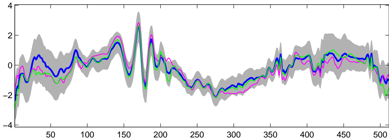
Estimated U_2(t) using G-WFMM: t_2 data, run 1
