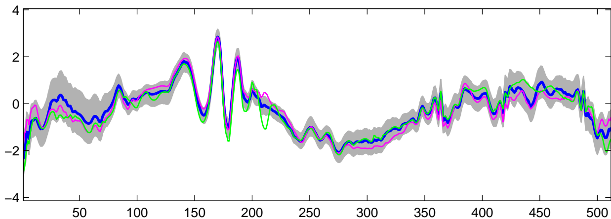
Estimated U_2(t) using R-WFMM: t_2 data, run 1
