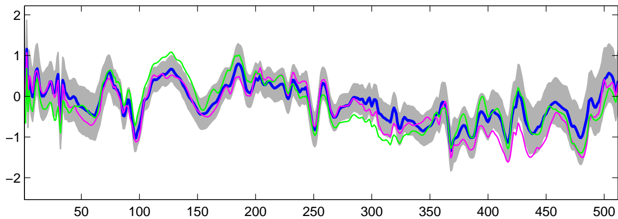
Estimated U_2(t) using R-WFMM: t_3 data, run 1
