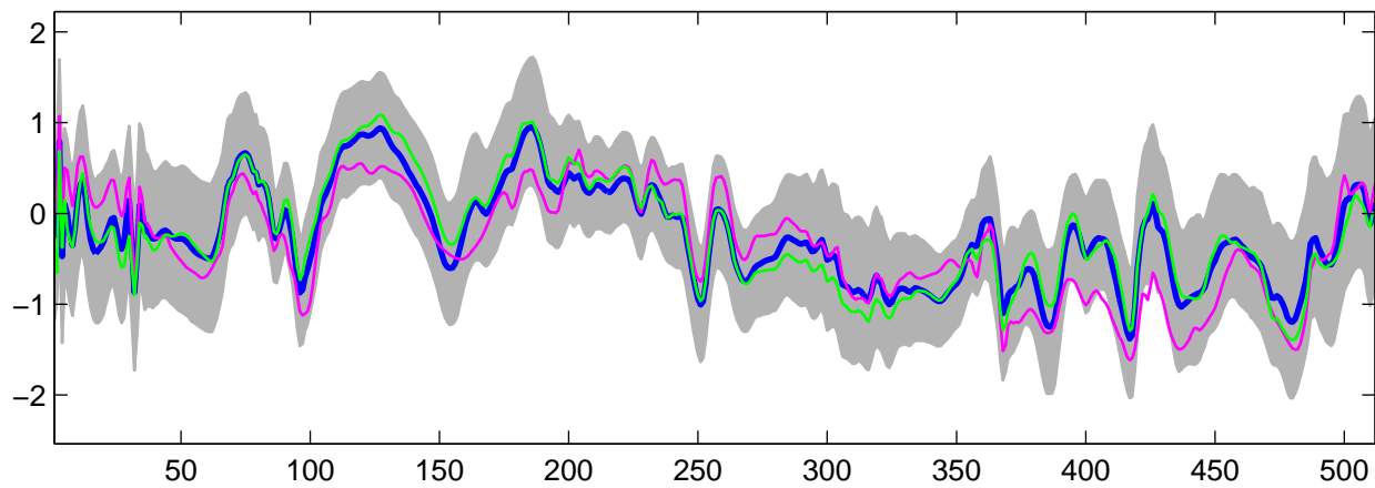
Estimated U_2(t) using G-WFMM: t_3 data, run 1
