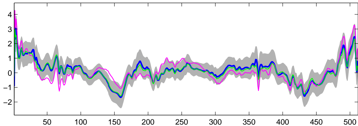
Estimated U_{30}(t) using G-WFMM: DE data, run 1
