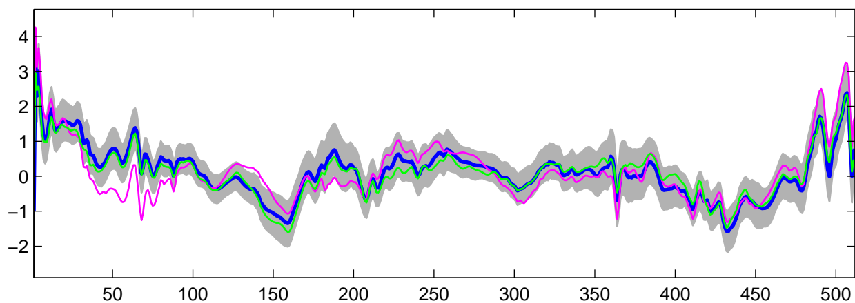
Estimated U_{30}(t) using R-WFMM: DE data, run 1
