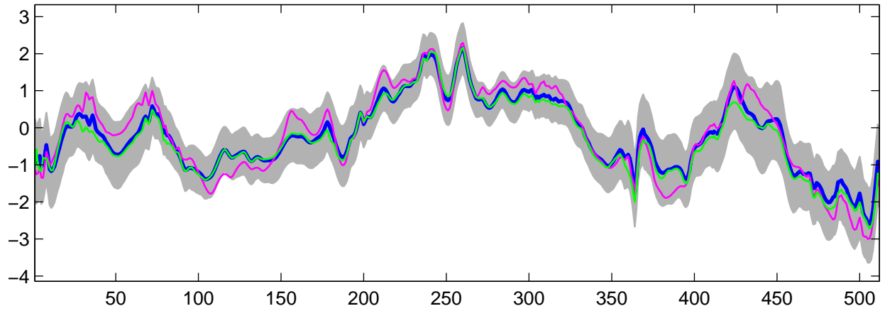
Estimated U_{30}(t) using G-WFMM: Normal data, run 1
