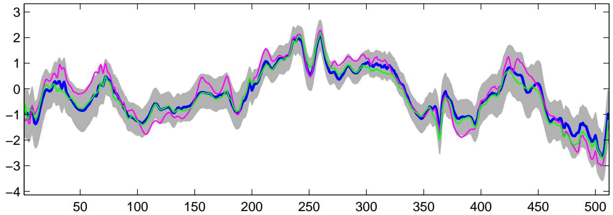
Estimated U_{30}(t) using R-WFMM: Normal data, run 1
