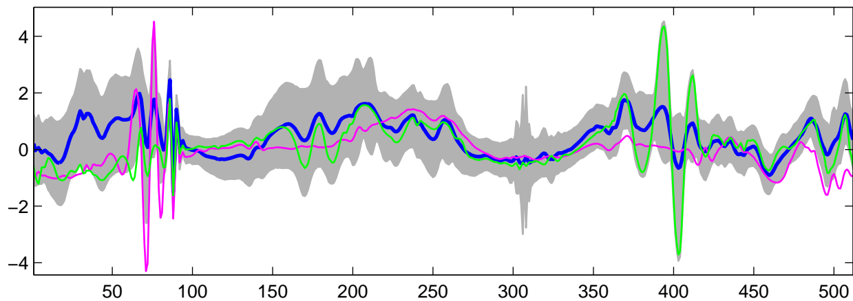
Estimated U_{30}(t) using G-WFMM: t_1 data, run 1
