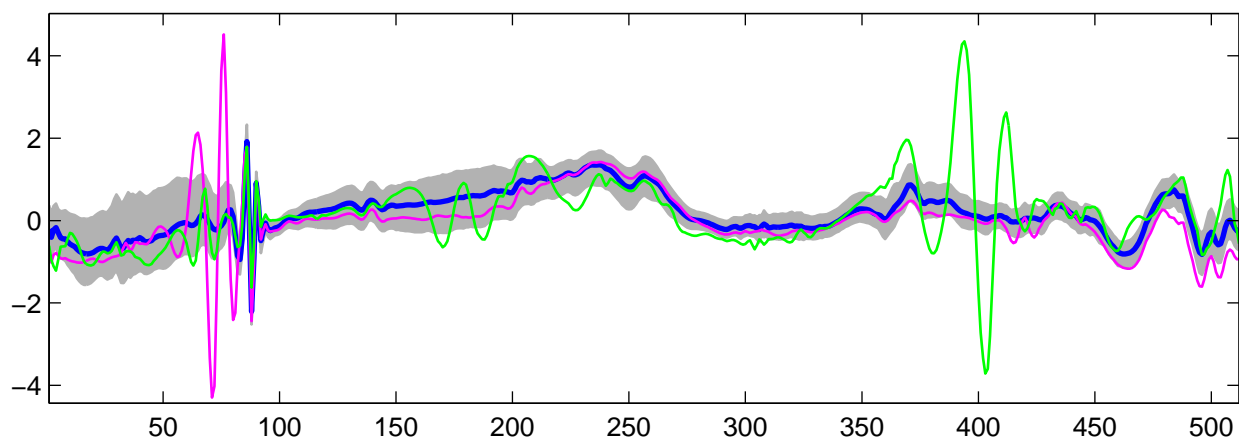
Estimated U_{30}(t) using R-WFMM: t_1 data, run 1
