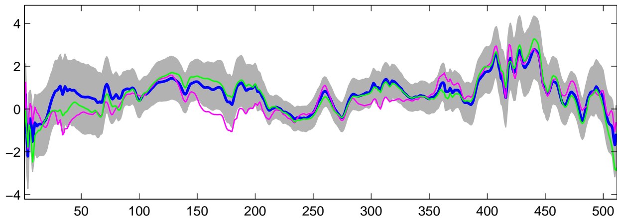
Estimated U_{30}(t) using G-WFMM: t_2 data, run 1
