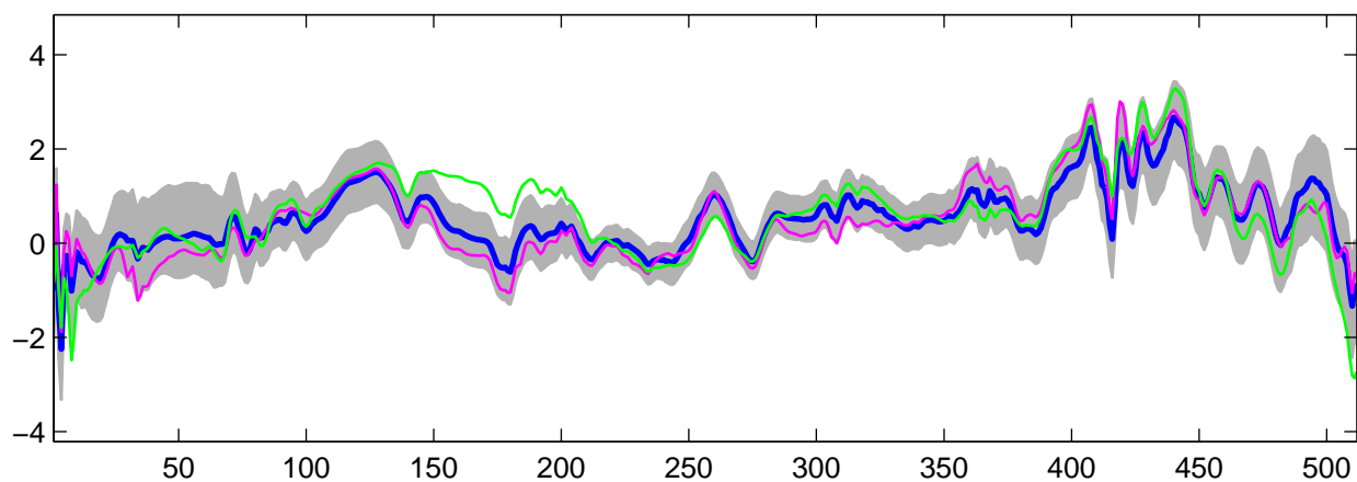
Estimated U_{30}(t) using R-WFMM: t_2 data, run 1
