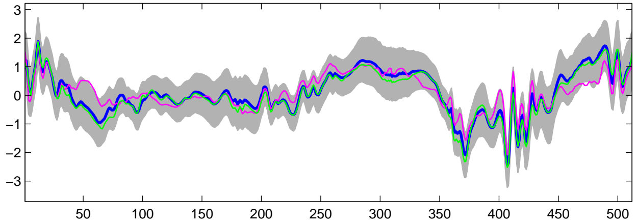
Estimated U_{30}(t) using G-WFMM: t_3 data, run 1
