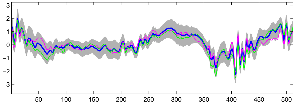
Estimated U_{30}(t) using R-WFMM: t_3 data, run 1
