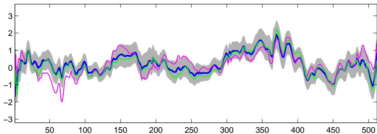
Estimated U_{31}(t) using R-WFMM: DE data, run 1
