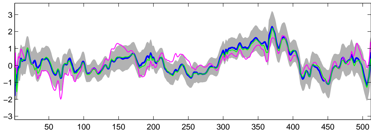
Estimated U_{31}(t) using G-WFMM: DE data, run 1
