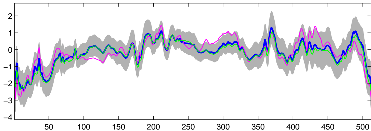
Estimated U_{31}(t) using G-WFMM: Normal data, run 1
