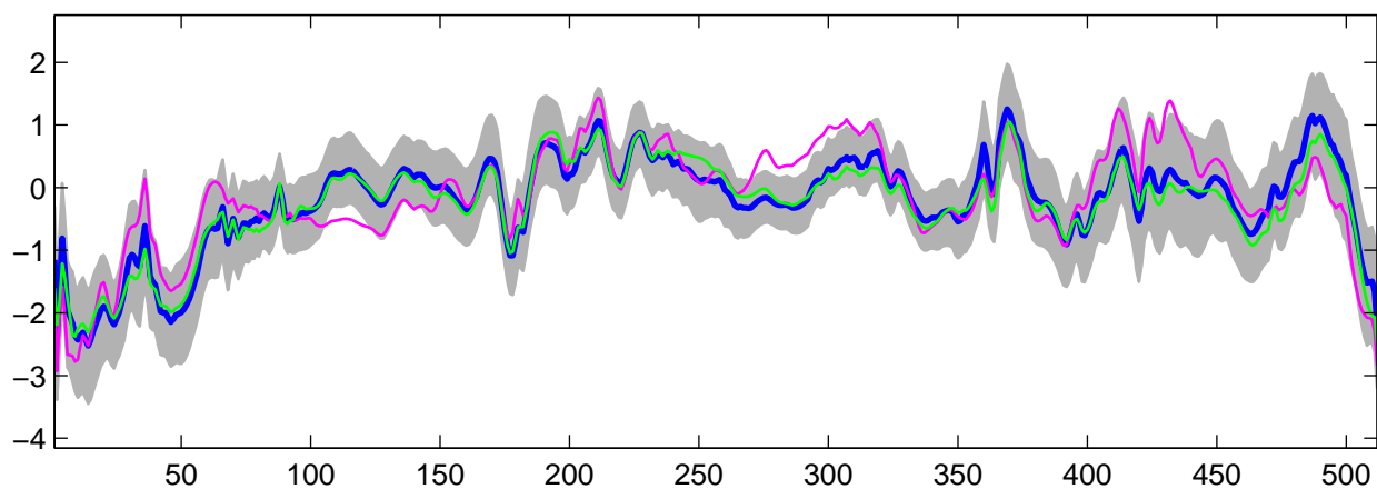
Estimated U_{31}(t) using R-WFMM: Normal data, run 1
