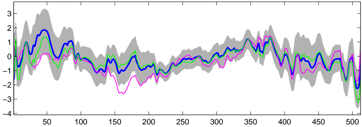
Estimated U_{31}(t) using G-WFMM: t_2 data, run 1
