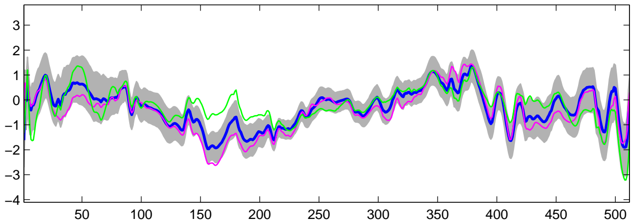
Estimated U_{31}(t) using R-WFMM: t_2 data, run 1
