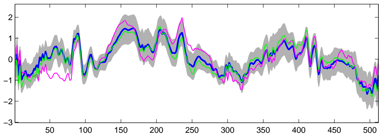
Estimated U_{32}(t) using R-WFMM: DE data, run 1
