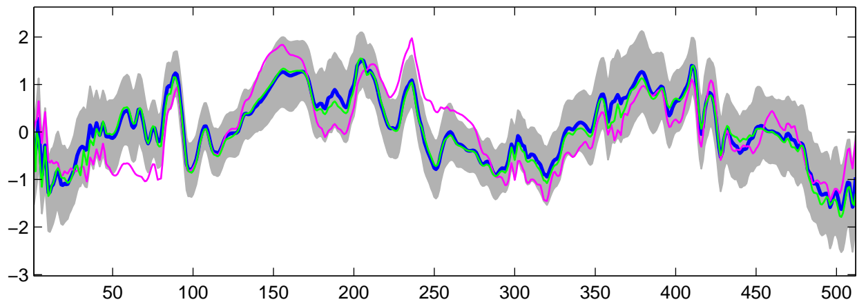
Estimated U_{32}(t) using G-WFMM: DE data, run 1
