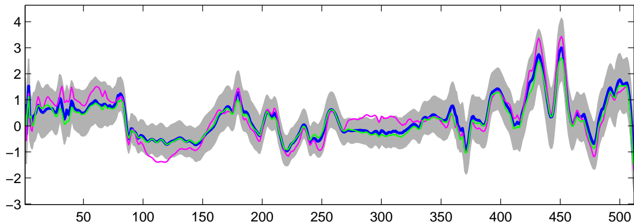
Estimated U_{32}(t) using G-WFMM: Normal data, run 1
