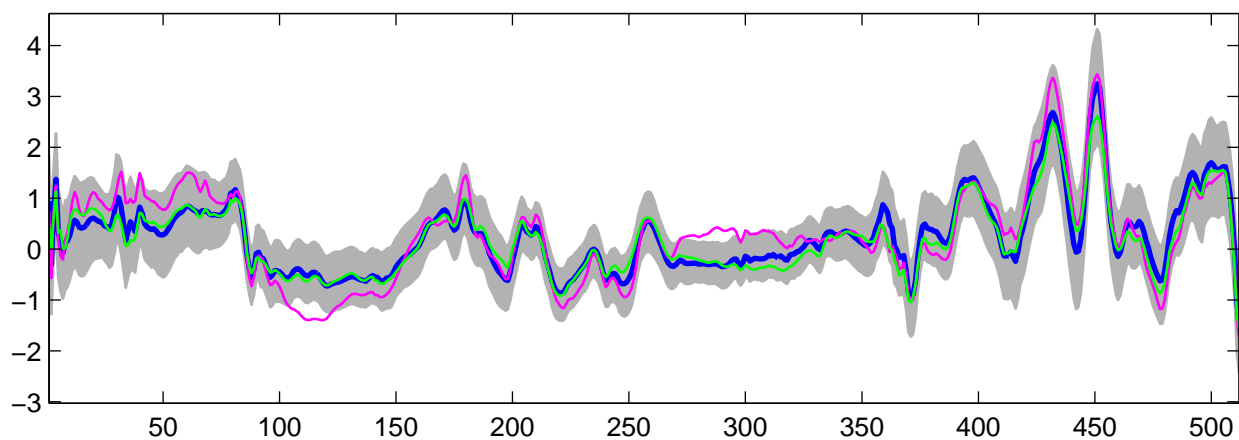
Estimated U_{32}(t) using R-WFMM: Normal data, run 1
