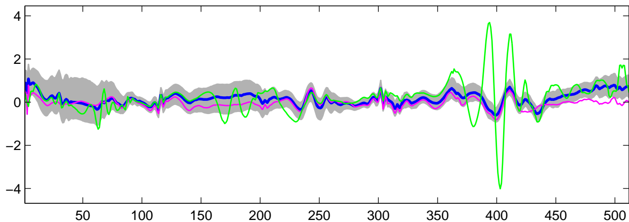
Estimated U_{32}(t) using R-WFMM: t_1 data, run 1
