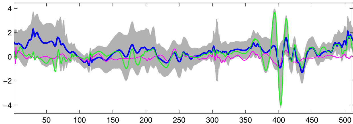
Estimated U_{32}(t) using G-WFMM: t_1 data, run 1
