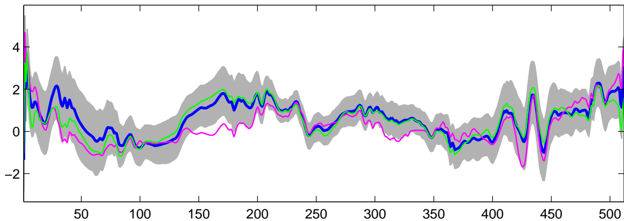
Estimated U_{32}(t) using G-WFMM: t_2 data, run 1
