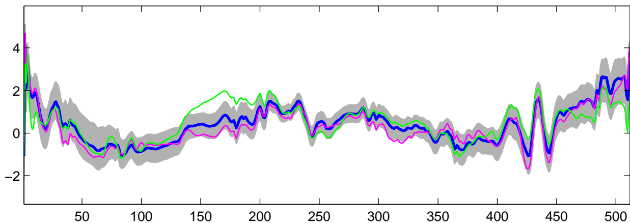
Estimated U_{32}(t) using R-WFMM: t_2 data, run 1
