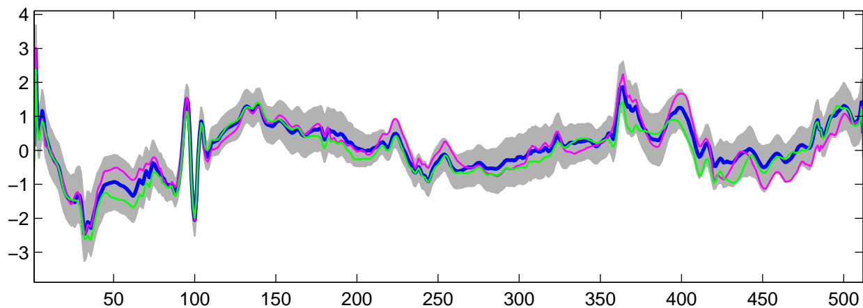
Estimated U_{32}(t) using R-WFMM: t_3 data, run 1
