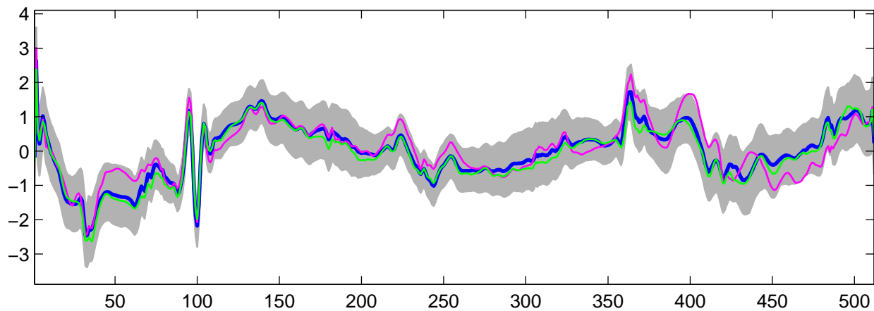
Estimated U_{32}(t) using G-WFMM: t_3 data, run 1
