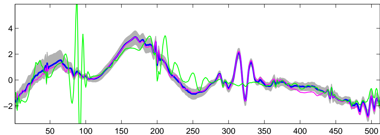
Estimated U_3(t) using R-WFMM: t_1 data, run 1
