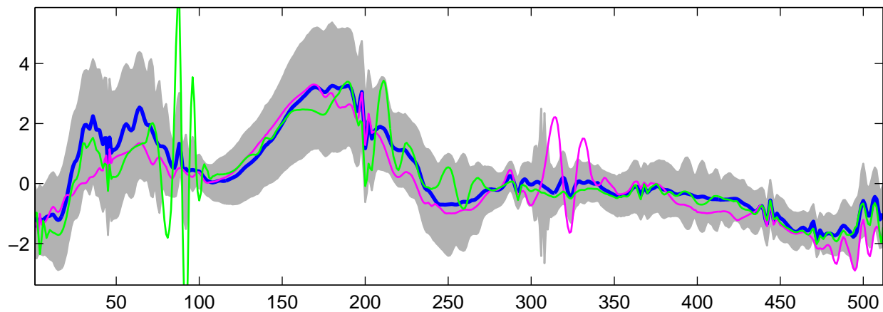
Estimated U_3(t) using G-WFMM: t_1 data, run 1
