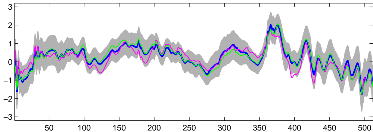
Estimated U_3(t) using G-WFMM: t_3 data, run 1
