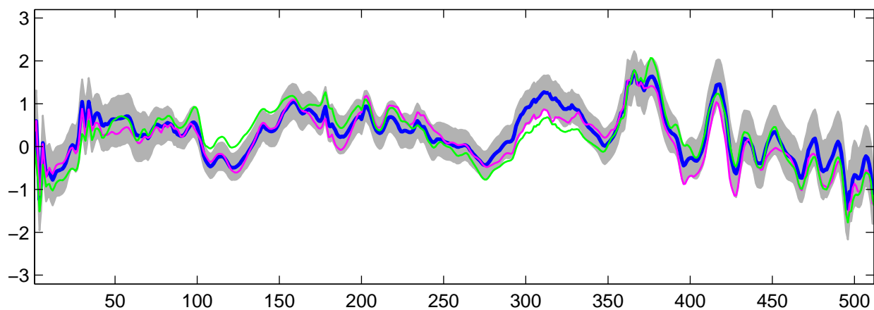
Estimated U_3(t) using R-WFMM: t_3 data, run 1
