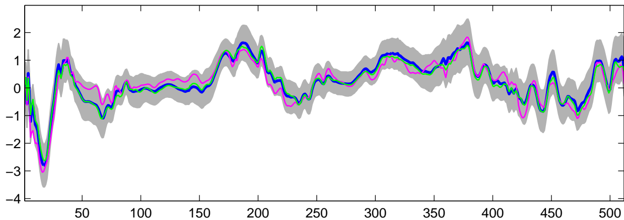
Estimated U_4(t) using G-WFMM: DE data, run 1
