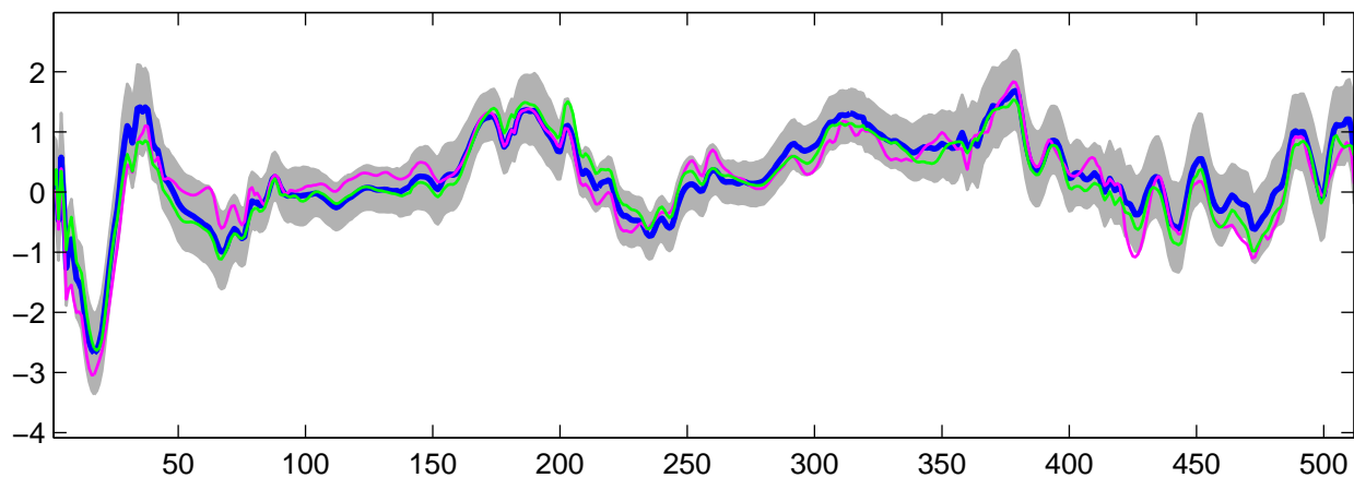
Estimated U_4(t) using R-WFMM: DE data, run 1
