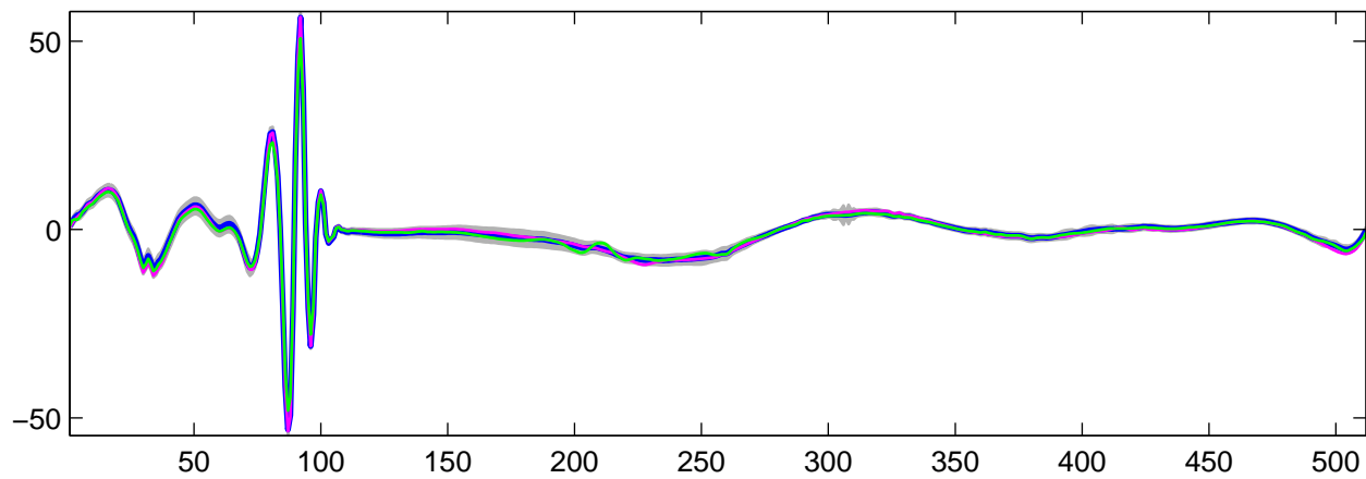
Estimated U_4(t) using G-WFMM: t_1 data, run 1
