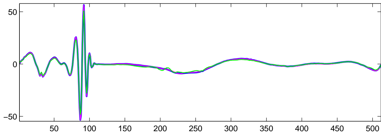
Estimated U_4(t) using R-WFMM: t_1 data, run 1
