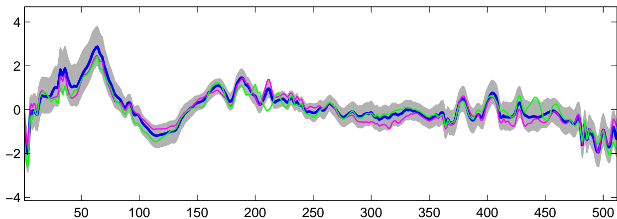
Estimated U_4(t) using R-WFMM: t_2 data, run 1
