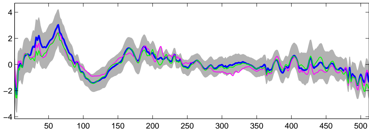
Estimated U_4(t) using G-WFMM: t_2 data, run 1
