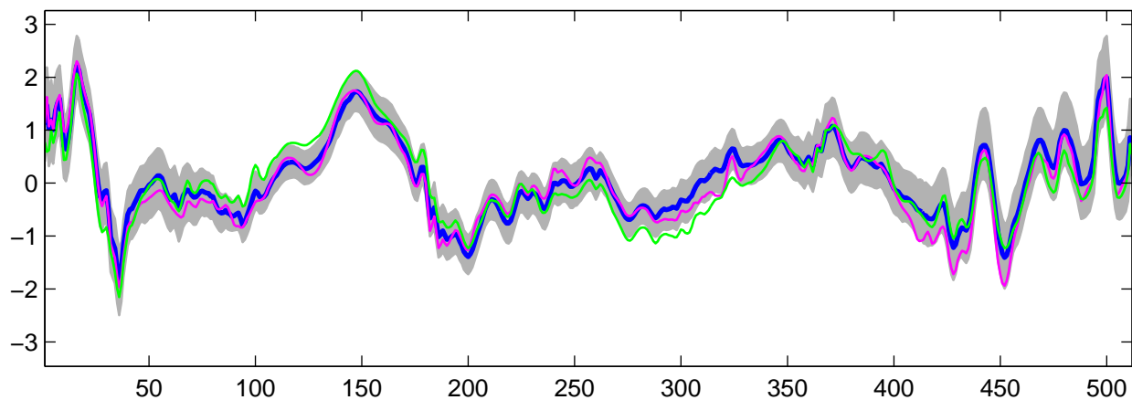
Estimated U_4(t) using R-WFMM: t_3 data, run 1
