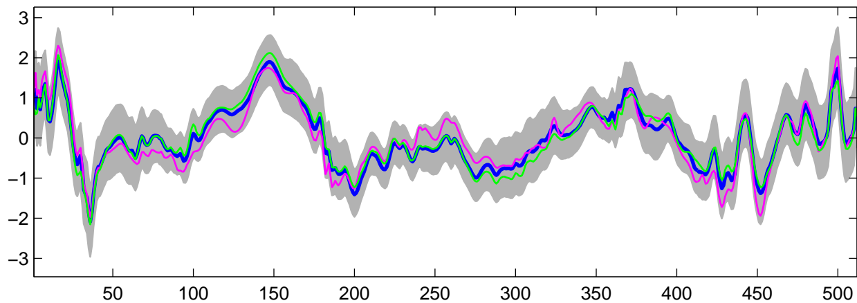
Estimated U_4(t) using G-WFMM: t_3 data, run 1
