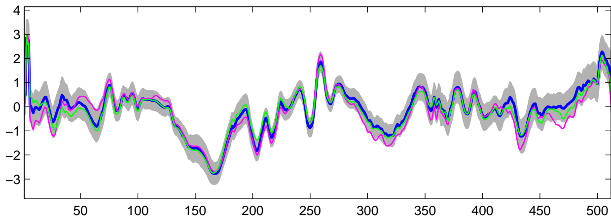
Estimated U_5(t) using R-WFMM: DE data, run 1
