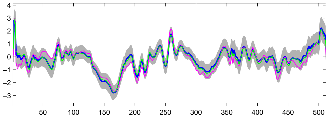
Estimated U_5(t) using G-WFMM: DE data, run 1
