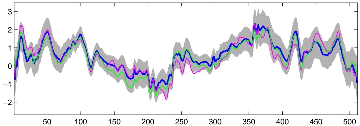
Estimated U_5(t) using R-WFMM: Normal data, run 1
