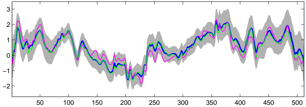
Estimated U_5(t) using G-WFMM: Normal data, run 1
