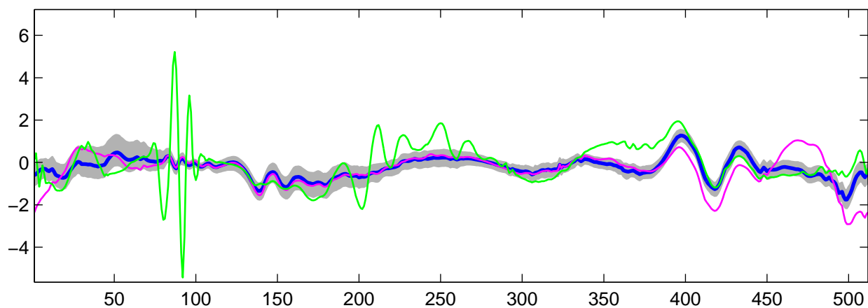
Estimated U_5(t) using R-WFMM: t_1 data, run 1
