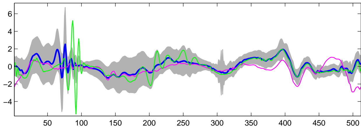
Estimated U_5(t) using G-WFMM: t_1 data, run 1
