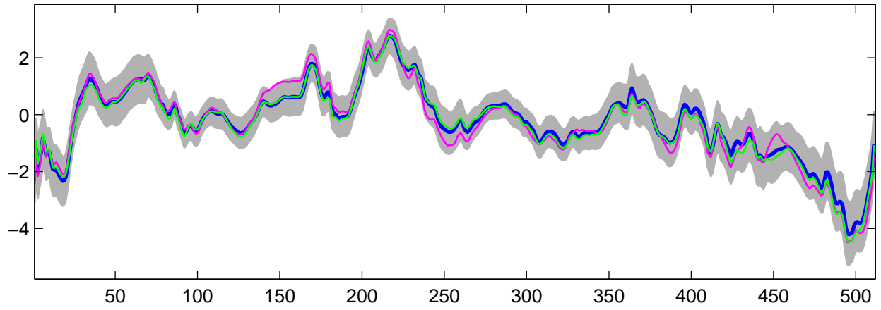
Estimated U_6(t) using G-WFMM: Normal data, run 1
