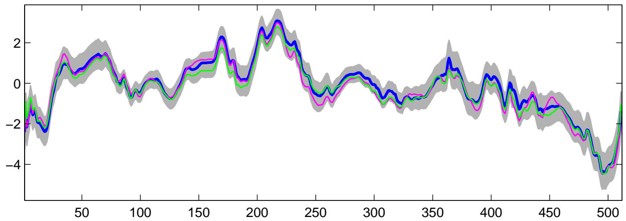
Estimated U_6(t) using R-WFMM: Normal data, run 1
