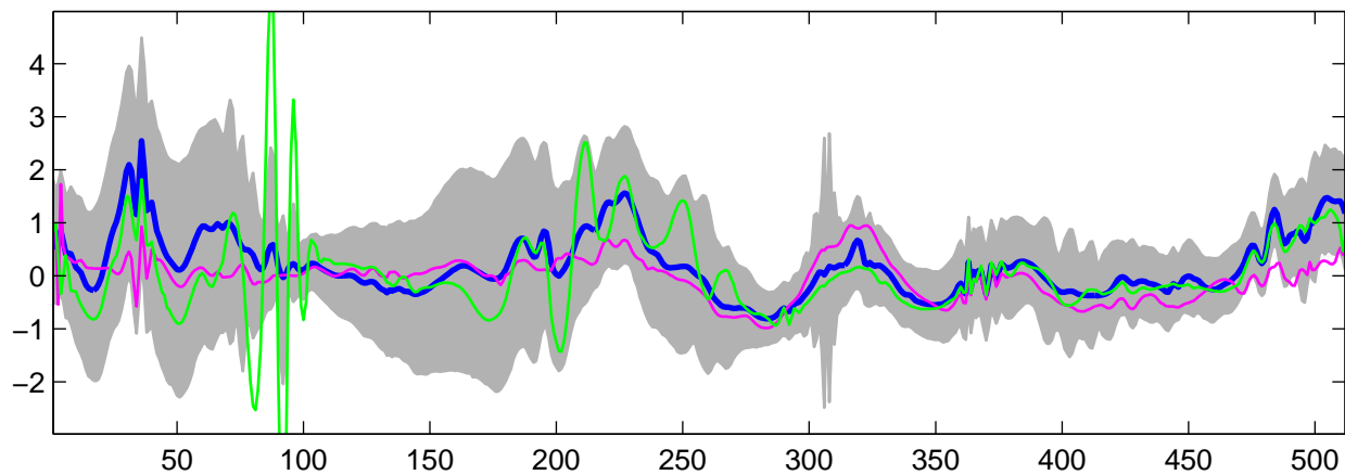
Estimated U_{\hat{\theta}}(t) using G-WFMM: t_1 data, run 1
