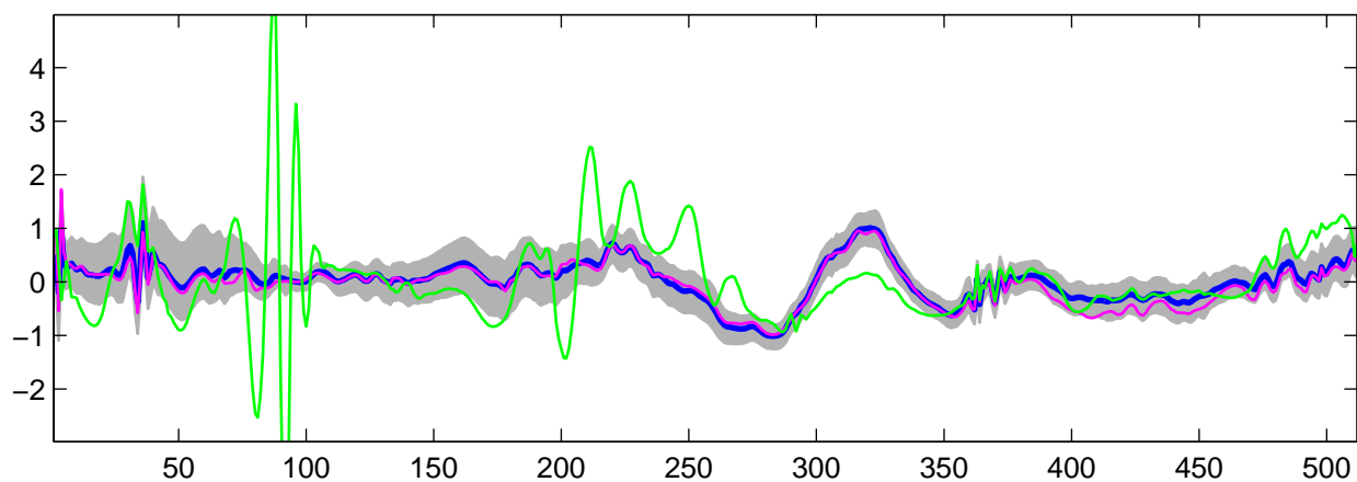
Estimated U_{\hat{\theta}}(t) using R-WFMM: t_1 data, run 1
