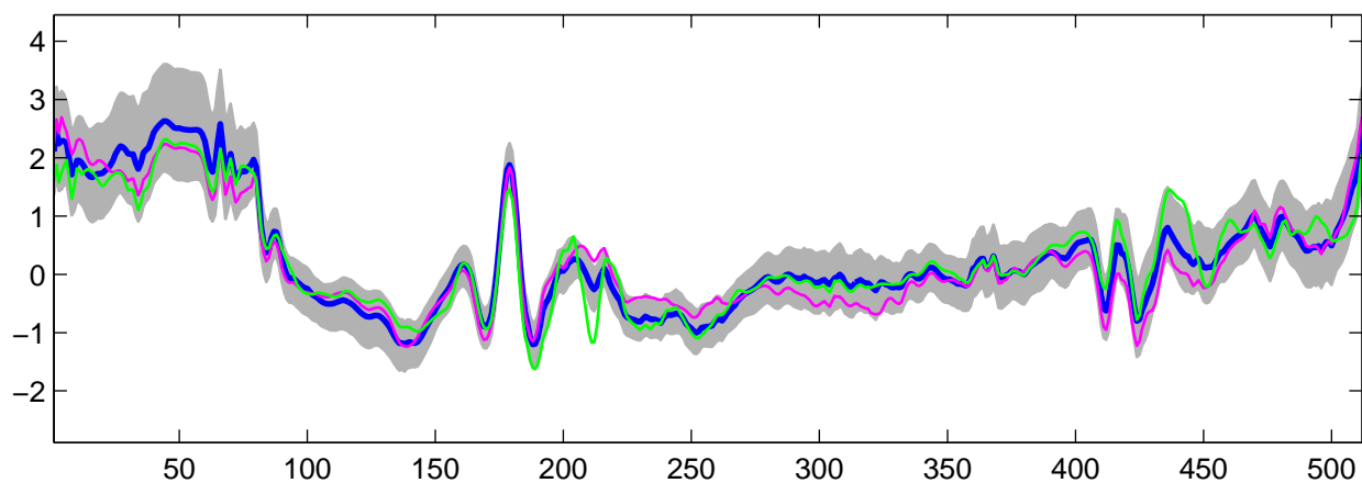
Estimated U_6(t) using R-WFMM: t_2 data, run 1
