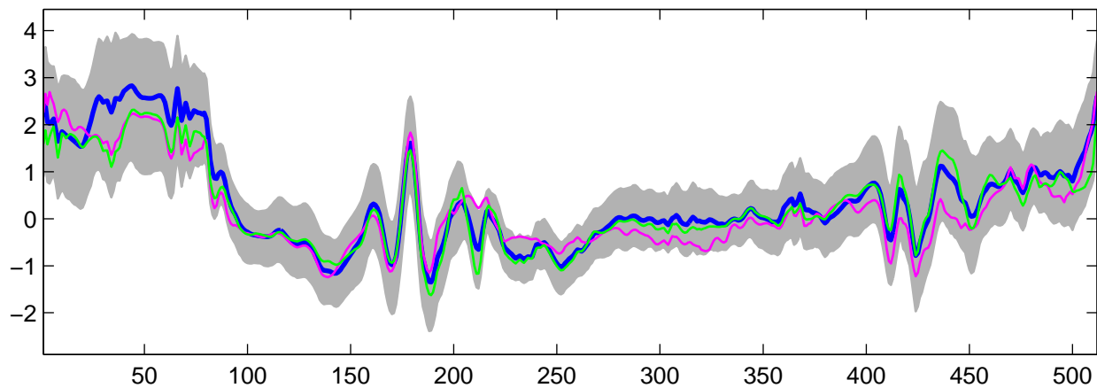
Estimated U_6(t) using G-WFMM: t_2 data, run 1
