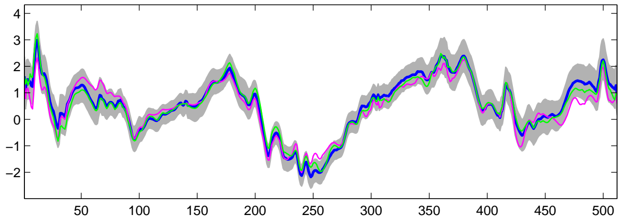
Estimated U_7(t) using R-WFMM: DE data, run 1
