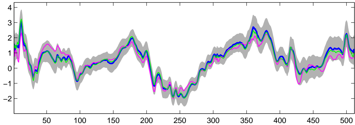
Estimated U_7(t) using G-WFMM: DE data, run 1
