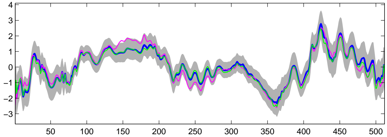
Estimated U_7(t) using G-WFMM: Normal data, run 1
