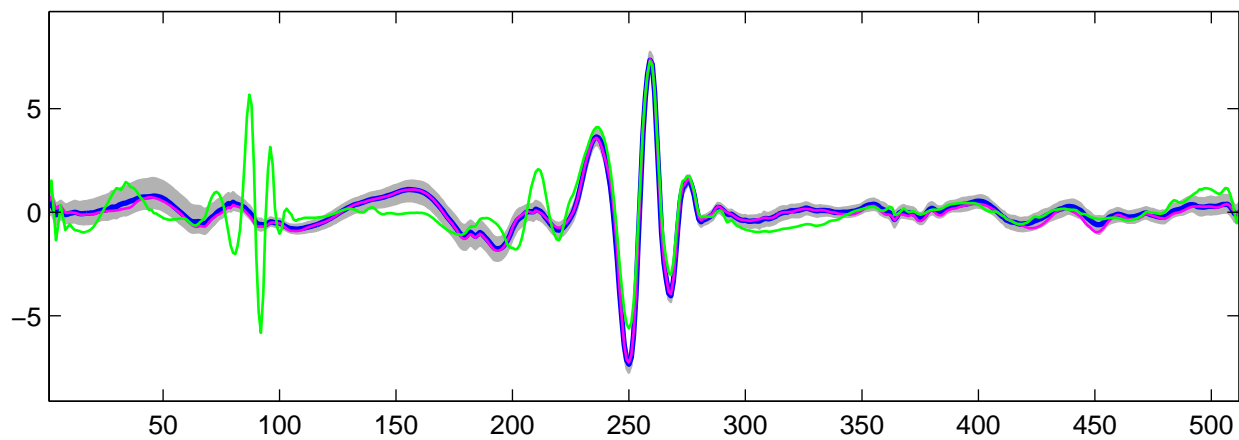
Estimated U_7(t) using R-WFMM: t_1 data, run 1
