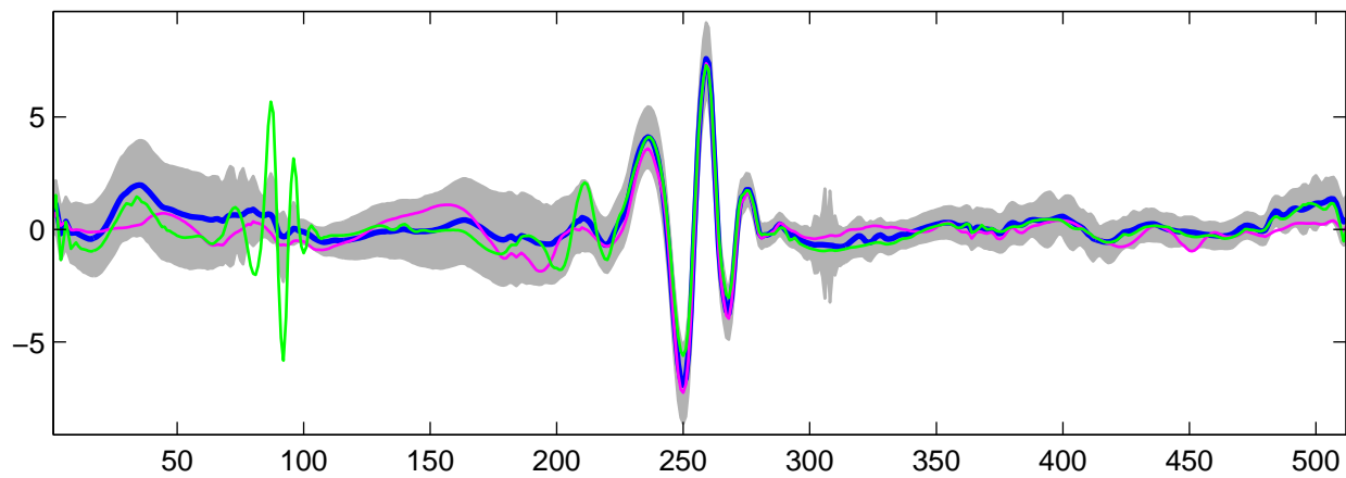
Estimated U_7(t) using G-WFMM: t_1 data, run 1
