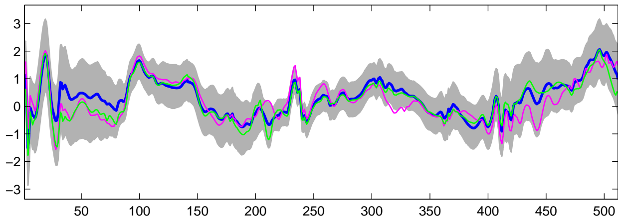
Estimated U_7(t) using G-WFMM: t_2 data, run 1
