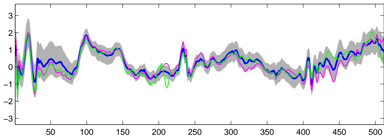
Estimated U_7(t) using R-WFMM: t_2 data, run 1
