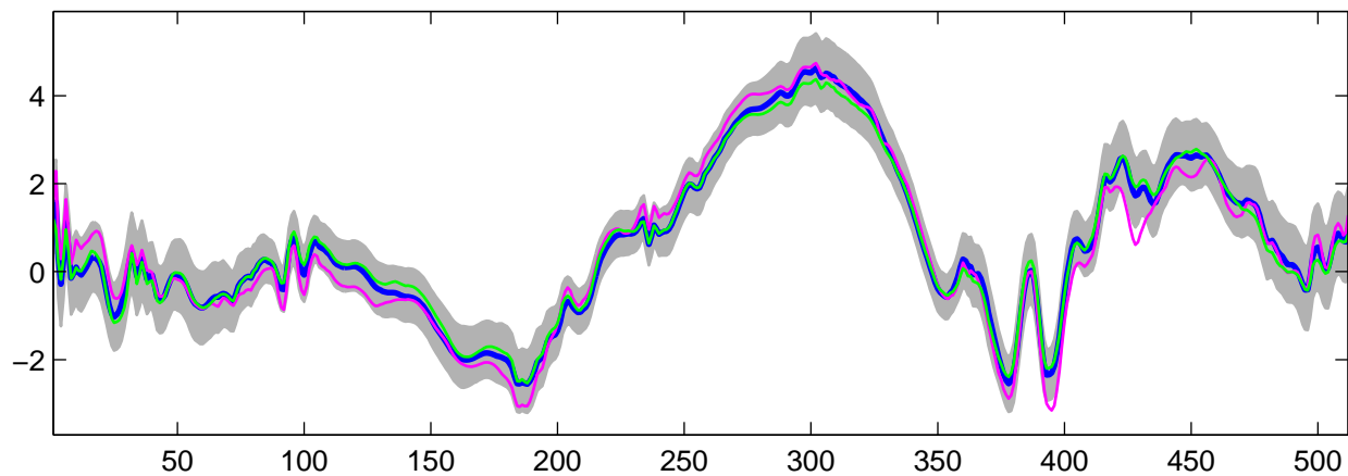
Estimated U_7(t) using G-WFMM: t_3 data, run 1
