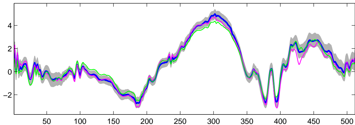
Estimated U_7(t) using R-WFMM: t_3 data, run 1
