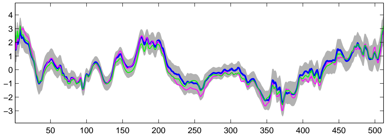
Estimated U_g(t) using R-WFMM: Normal data, run 1
