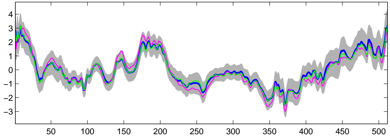
Estimated U_g(t) using G-WFMM: Normal data, run 1
