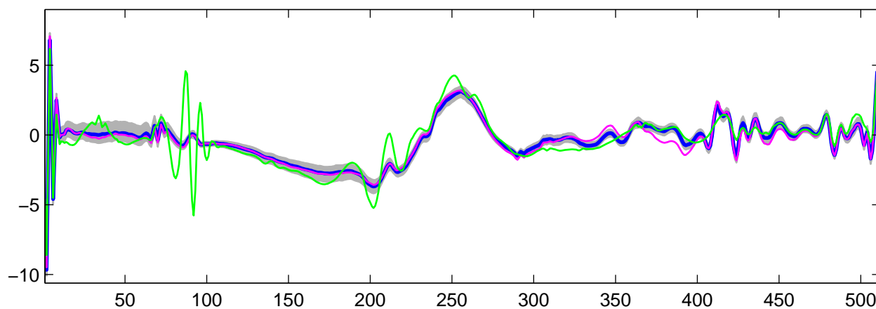
Estimated U_8(t) using R-WFMM: t_1 data, run 1
