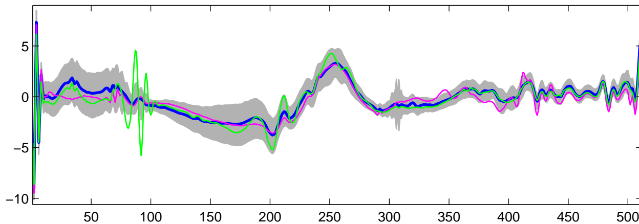
Estimated U_8(t) using G-WFMM: t_1 data, run 1
