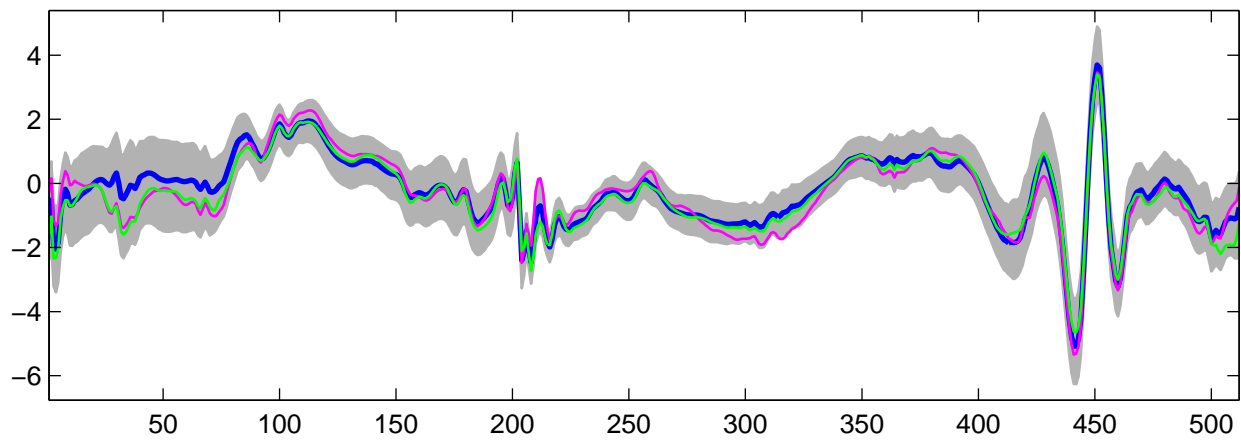
Estimated U_8(t) using G-WFMM: t_2 data, run 1
