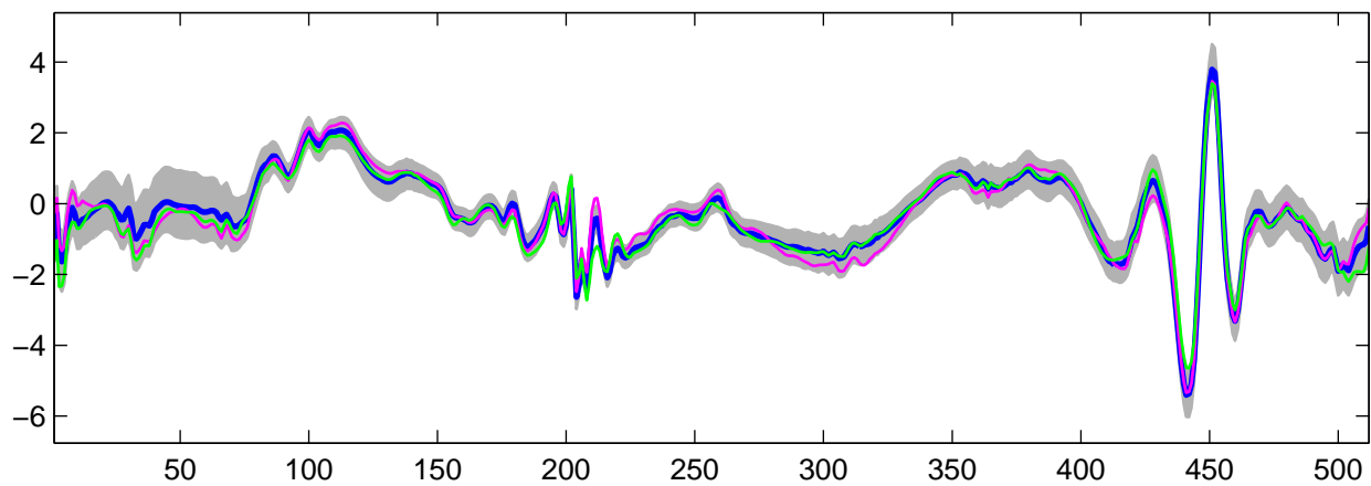
Estimated U_8(t) using R-WFMM: t_2 data, run 1
