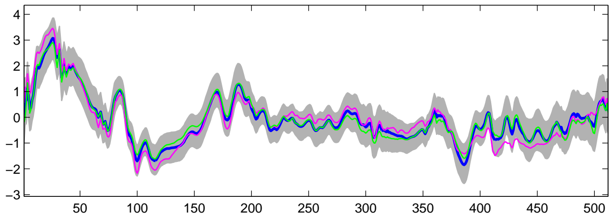
Estimated U_8(t) using G-WFMM: t_3 data, run 1
