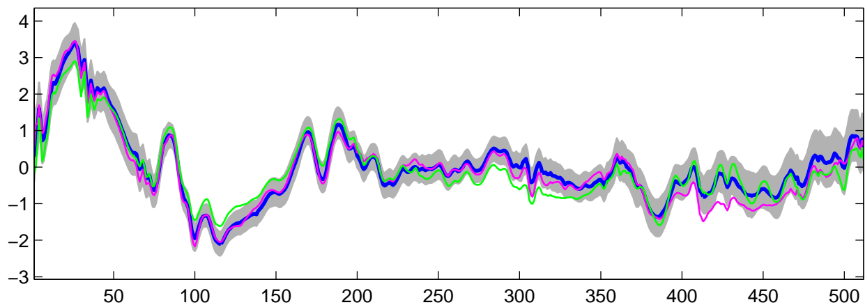
Estimated U_8(t) using R-WFMM: t_3 data, run 1
